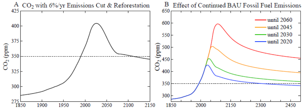
Fig. 4. (A) Atmospheric CO 2 if fossil fuel emissions are cut 6%/year beginning in 2013 and 100 GtC reforestation drawdown occurs in 2031-2080, (B) effect of delaying onset of emissions reduction.
