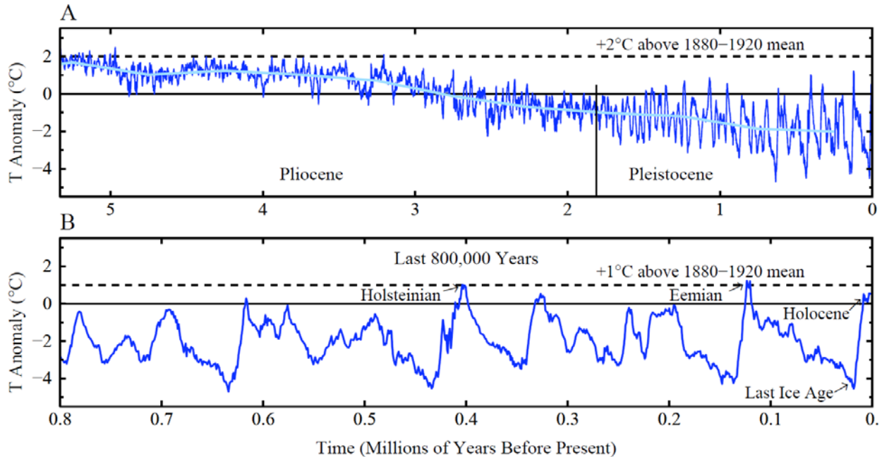
Fig. 2. Global temperature relative to 1880-1920 in (A) past 5,300,000 and (B) past 800,000 years (32).
